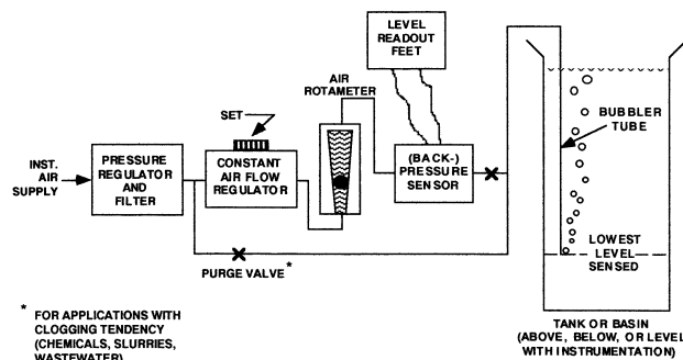
FUNCTIONAL DIAGRAM
