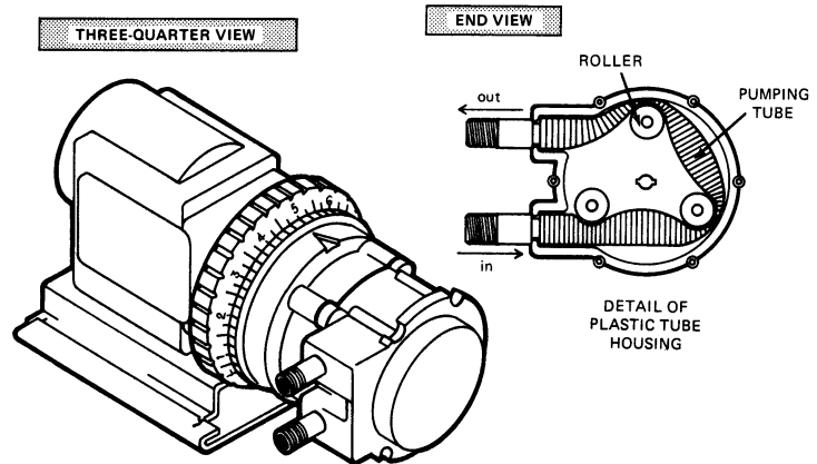
Peristaltic Pump
