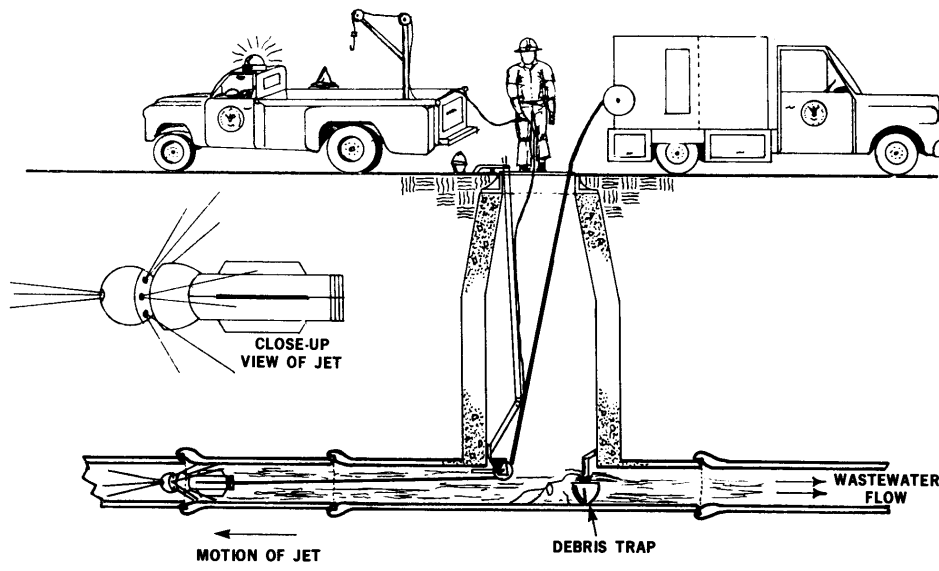
Jet Cleaner Operation
