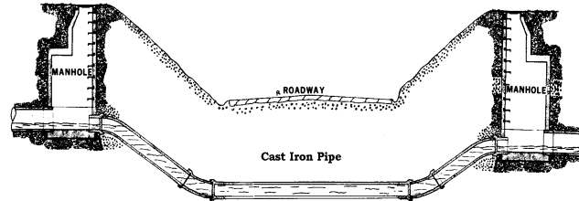
Inverted Siphon
