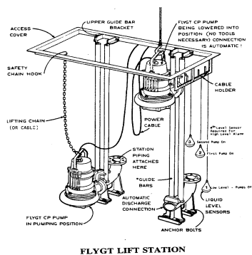
FLYGT LIFT STATION Wet Well Lift Station
