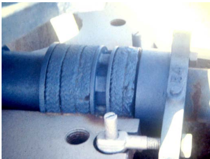
Stuffing Box on a Horizontal Split Case Pump
