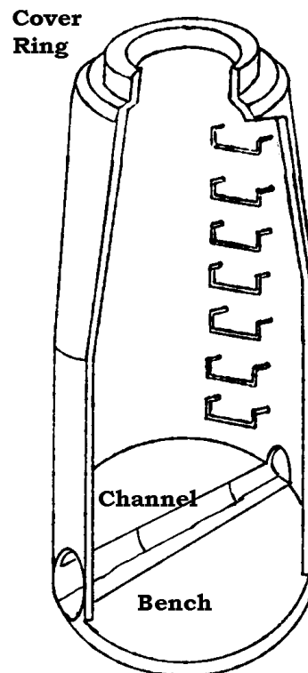
Typical Manhole
