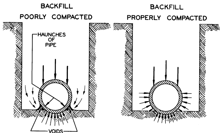
VOIDS, OR POORLY COMPACTED BACKFILL AT HAUNCHES, CAUSES SUBSIDIENCE OF THE BACKFILL AT SIDES OF PIPE AND SUBSEQUENT LOSS OF SIDE SUPPORT.
