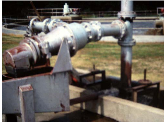
Grit is separated and deposited in a grit classifier (left side) and the water is returned as a sidestream (right side).
